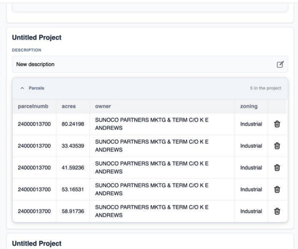
Меню "Projects"
